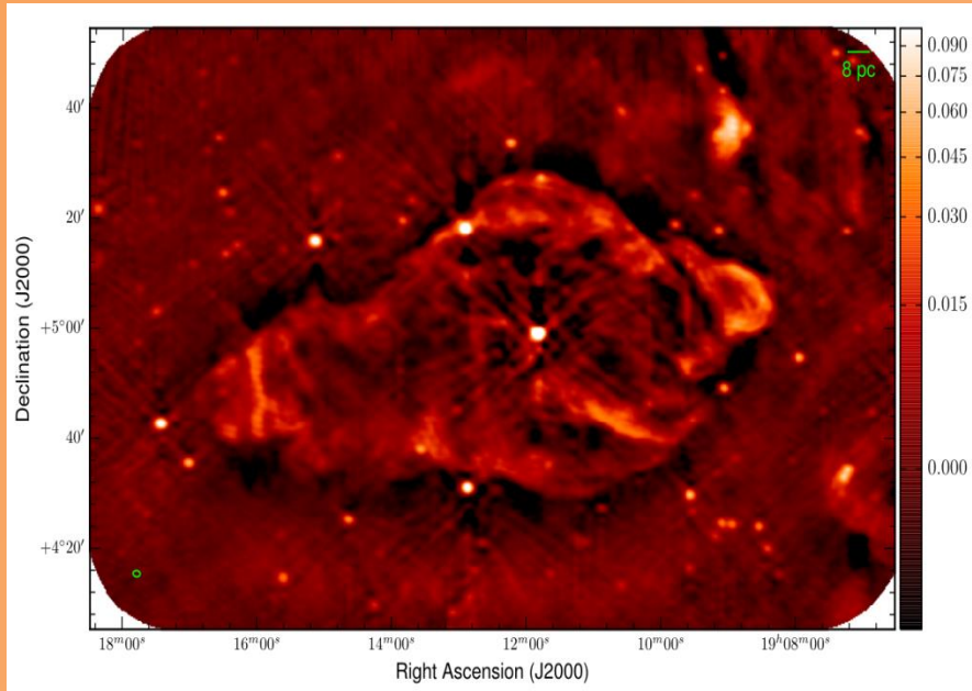
Stokes I from 1.4-3GHz ( Farnes et al. 2017)
