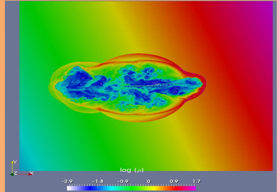
Output (density) from simulations
